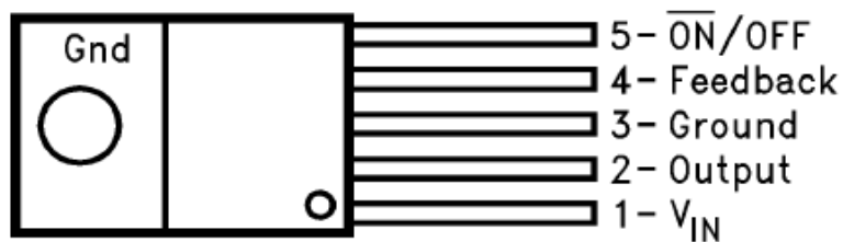
Figure: 3 pin out of LM2576
