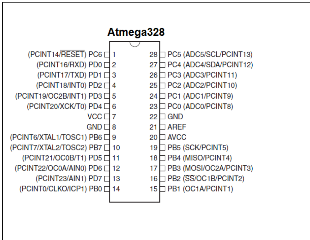
Figure 2: pin out of ATmega 328
